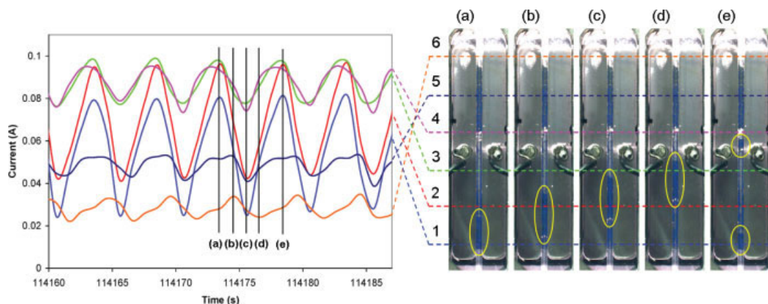
Figure 16. Spatio-temporal correlation of local current and water slugs in the vertical SAPC fuel cell with the flows against gravity (V-ii).
