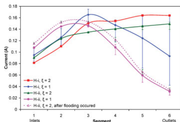
Figure 11. Steady-state current density profiles for the SAPC \text{H}_2/\text{O}_2 fuel cell in two horizontal configurations: the cathode facing down (H-i) and the cathode facing up (H-ii); and two feed stoichiometries: \xi_1 and \xi_2 .
