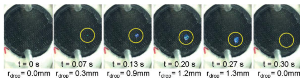
Figure 5. Series of photos showing drop formation and detachment from the surface of a carbon cloth GDL under an applied hydraulic pressure of 170 mm \text{H}_2\text{O} .
